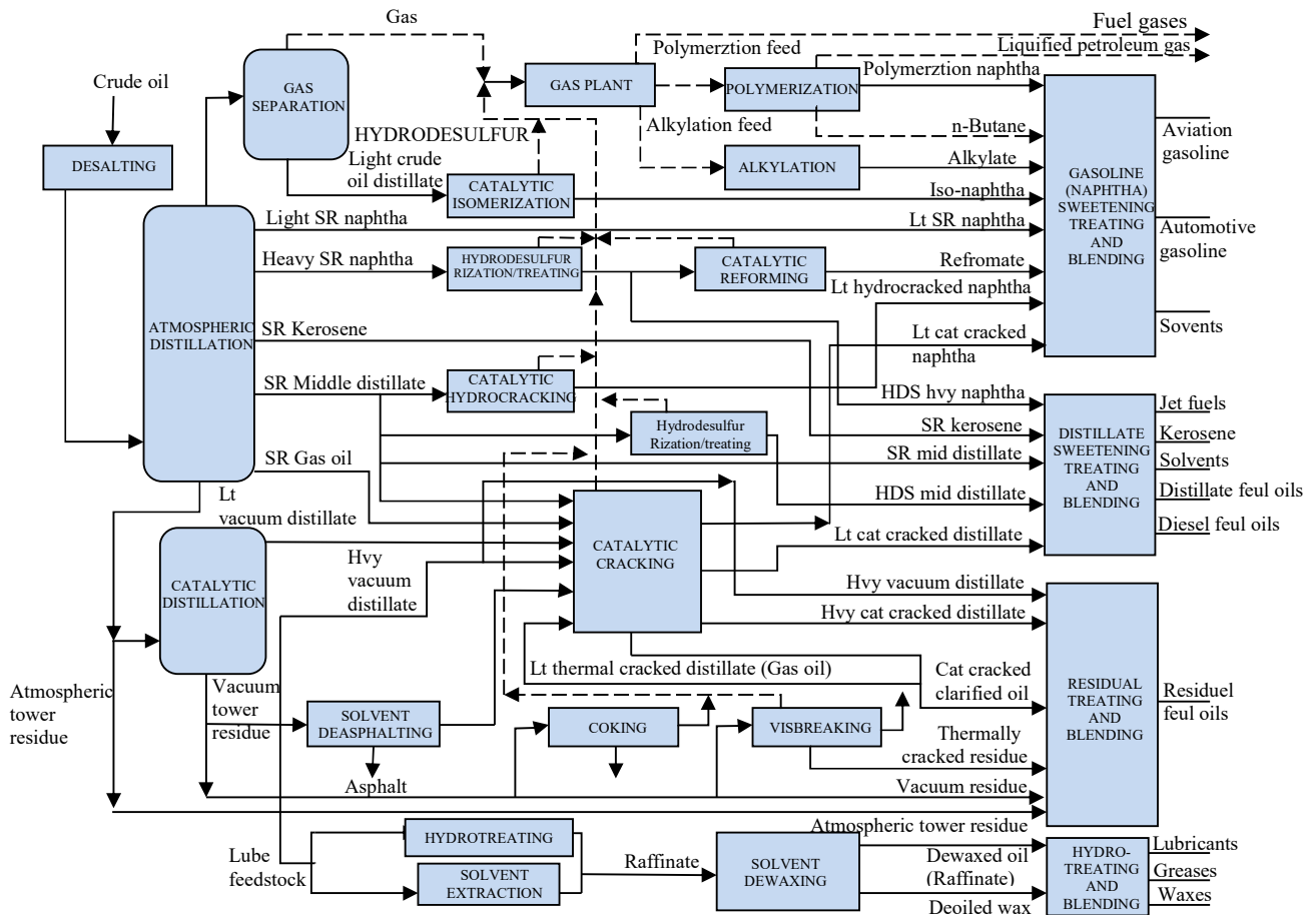
Figure 1 : refinery process
