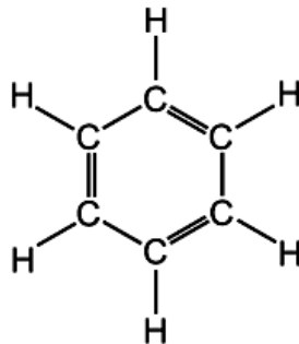
Figure 4 : example of aromatics; Benzene
