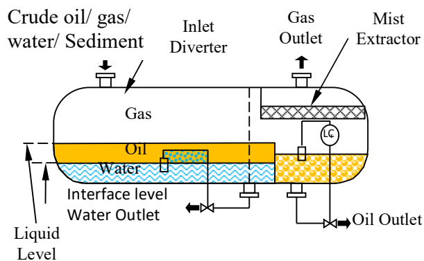
Figure 7 : field separator
