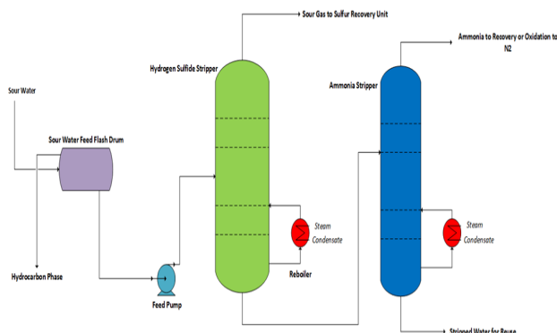
Figure 3 – Typical Arrangement for Sour Water Stripping Unit with Two Towers
