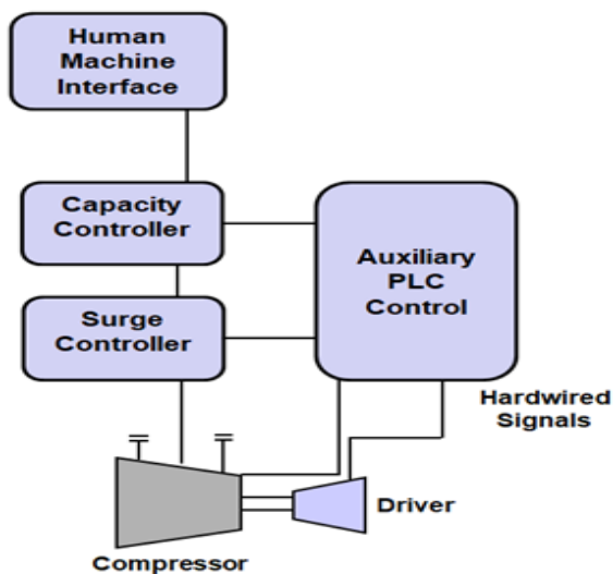
Figure 5. Compressor System with Interfaces
