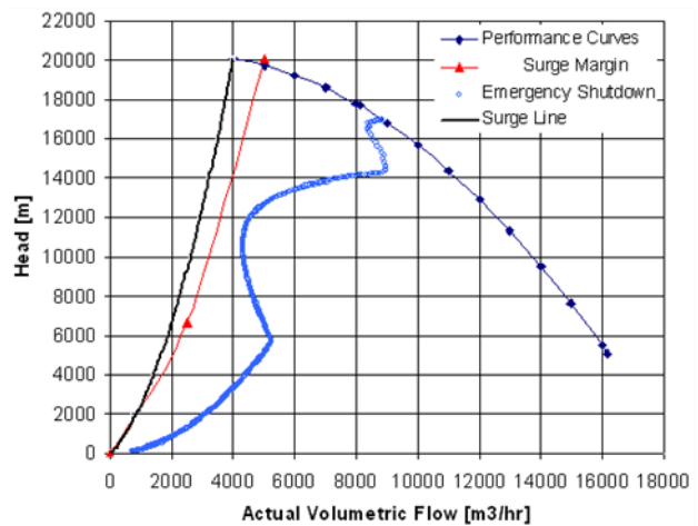
Figure 4. Surge Avoided with Hot Gas Recycle
