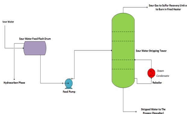
Figure 2 – Typical Arrangement for Sour Water Stripping Unit with Single Tower
