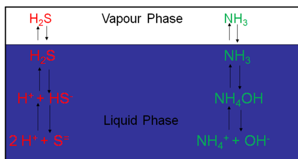
Figure 1 – Phase Equilibrium in Sour Water Stripping Process
