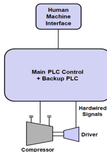
Figure 6. Compressor System with Integrated Interfaces
