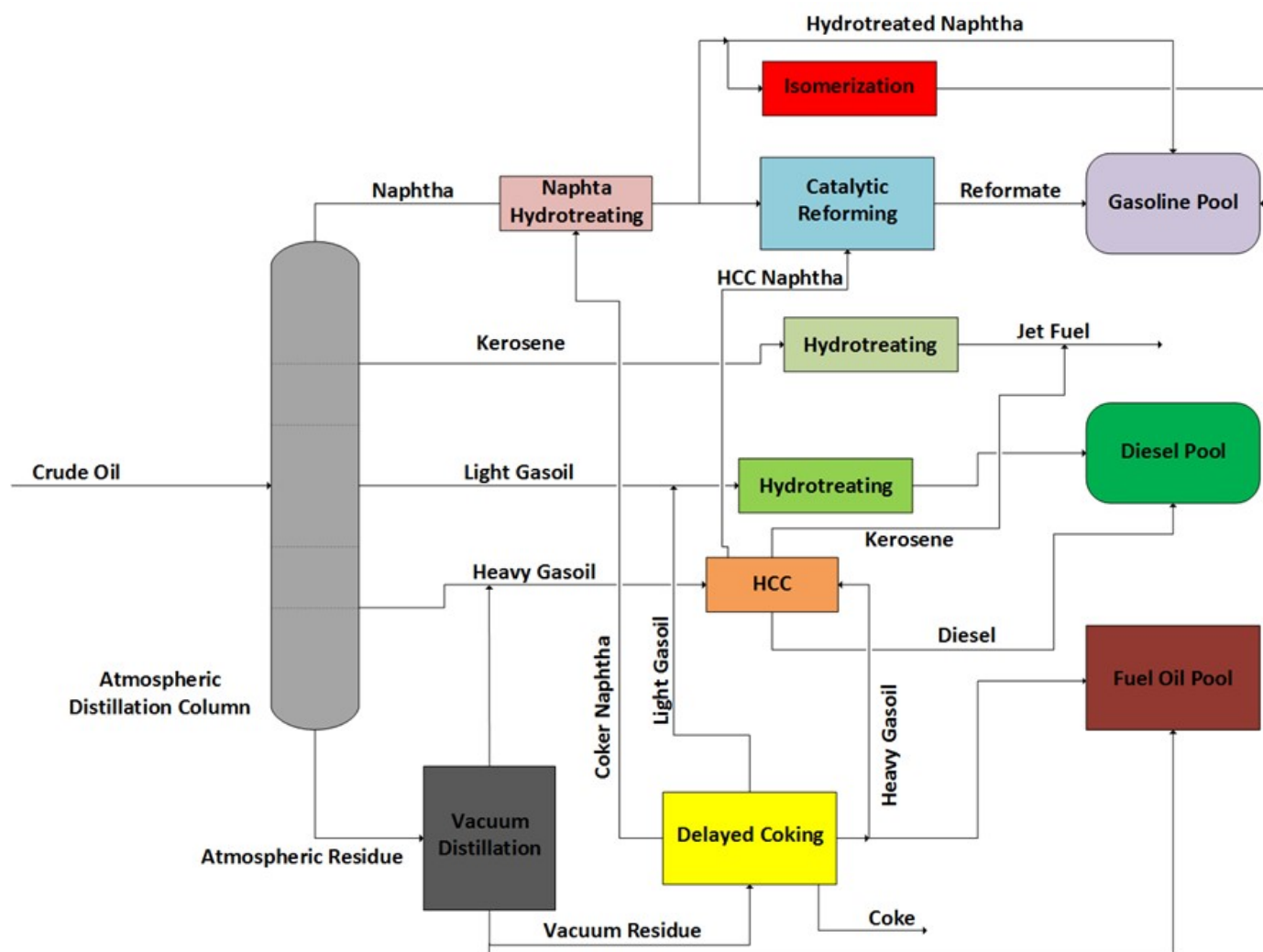
Figure 2 – Process Arrangement for a Typical Refinery Operating Under Coking/Hydrocracking Configuration
