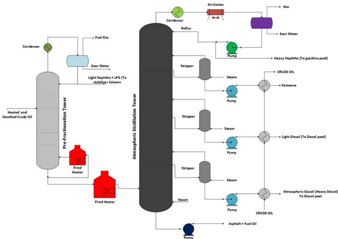
Figure 1 – Typical Process Configuration to a Refinery with “Topping” Refining Configuration
